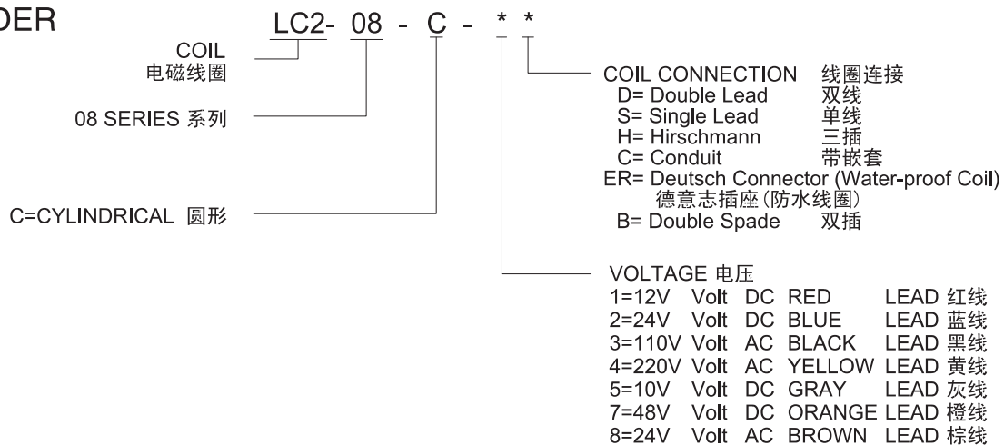
Model:LC2-08-C-*ER Deutsch Connector (Water-proof Coil)
