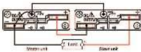
Series Connection
