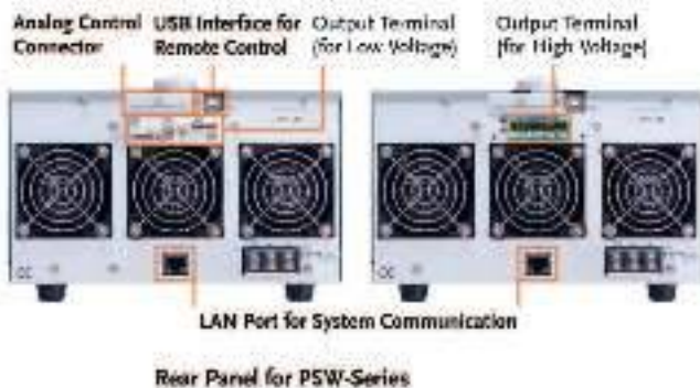
Rear Panel for PSW-Series
