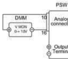
External DMM Monitoring of the Output Voltage
