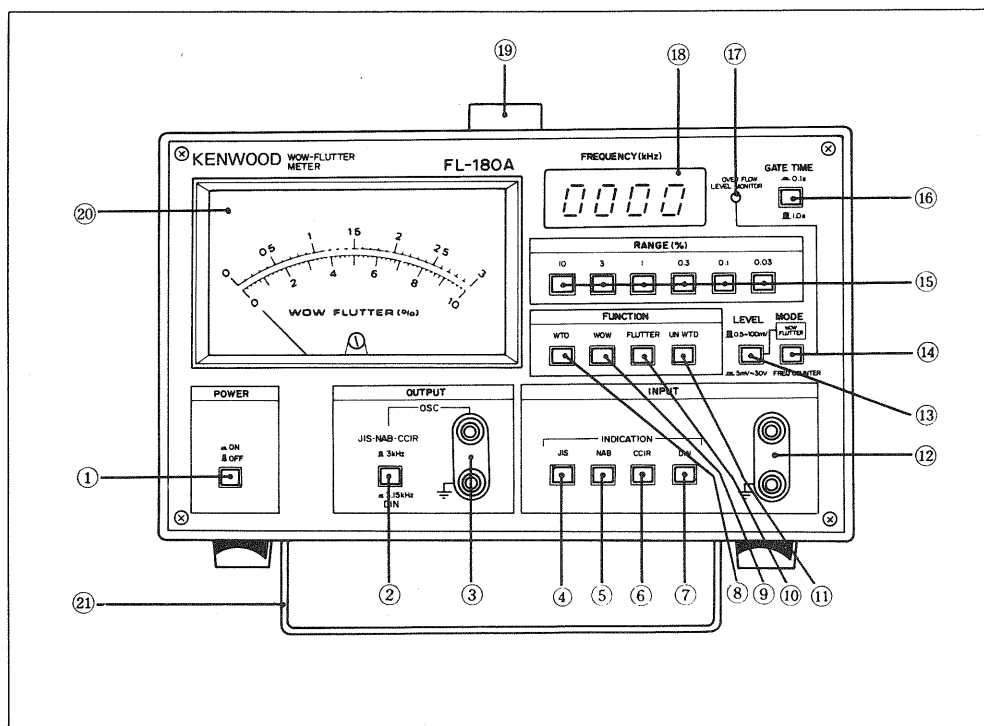
Fig. 1 Front panel
