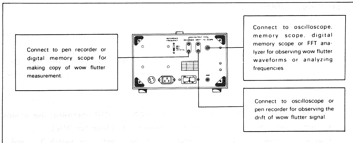
Fig 5 Out put terminal on rear panel
