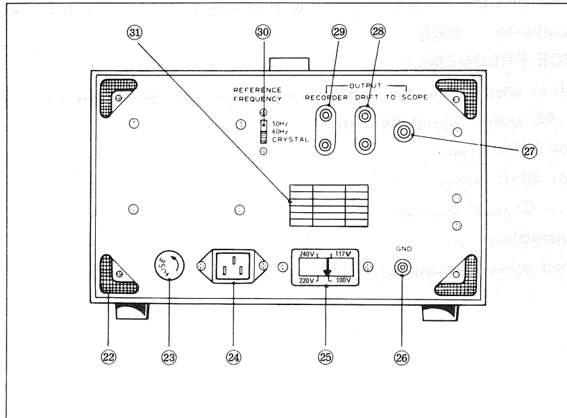
Fig. 3 Rear panel
