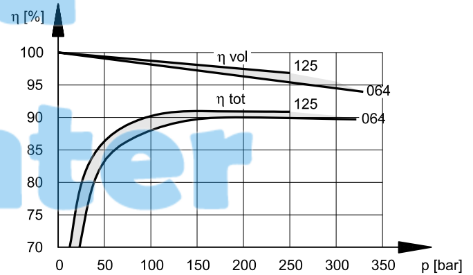
VOLUMETRIC AND TOTAL EFFICIENCIES
