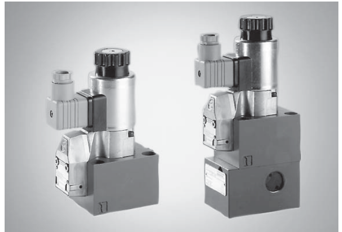
Type M-3SEW 10 D U 1X/...K4/... with plug-in connector (separate order)
